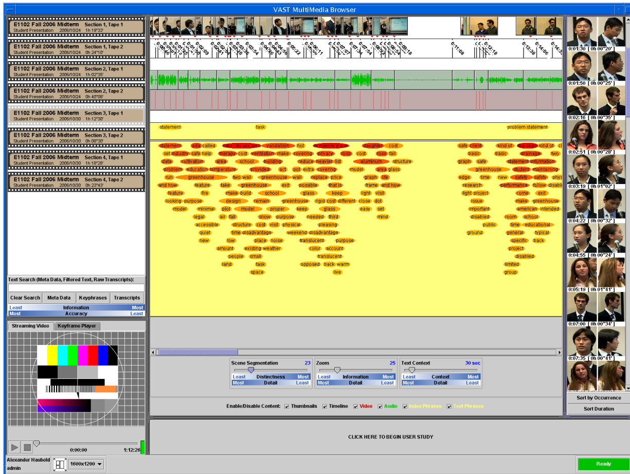
Figure 4: VAST MM (Video Audio Structure Text MultiMedia) browser. Featured on the left are videos from the course. Upon selecting a video, the video summary and streaming video is loaded. The summary features thumbnail keyframes, which enlarge on mouse-overs, speaker segmentation UI, video segmentation UI, keyword and key phrase UIs, a visual speaker index, and streaming and keyframe players.
